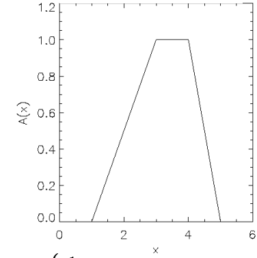
trapezoidal function
