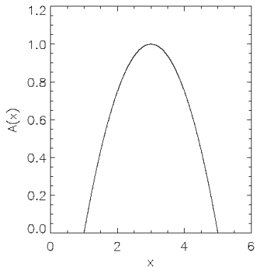
paraboloidal function
