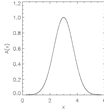
gaussoid function
