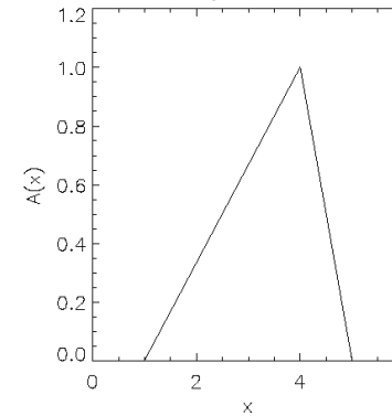
triangle function
